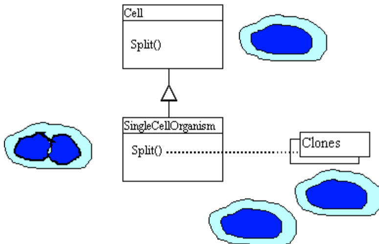
Figure 4: Object Diagram for Prototype using Cell Division Example
